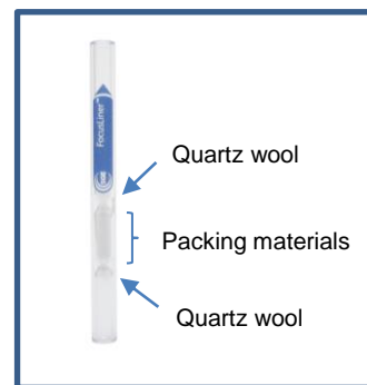
Packed GC Glass Insert A (for Agilent GC)
